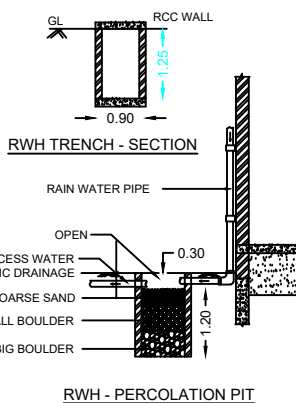
RWHP - PERCOLATION PIT
