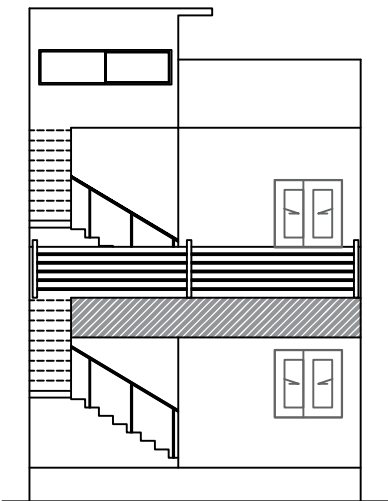
FRONT ELEVATION
