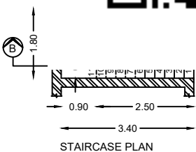
STAIRCASE PLAN
