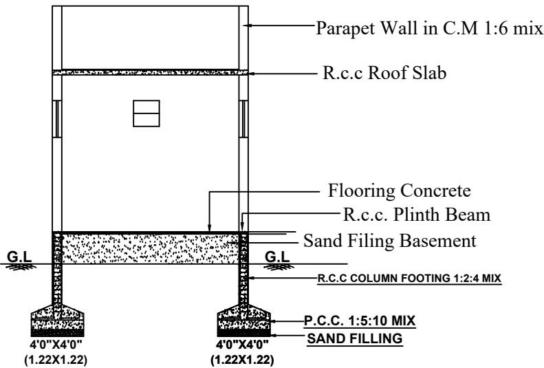
. SECTION OF TOILET.
