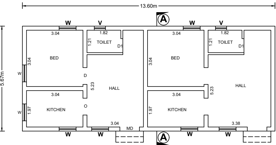
. PLAN OF STAFF QUARTERS.
