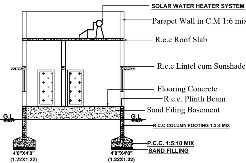
. SECTION OF STAFF QUARTERS.
