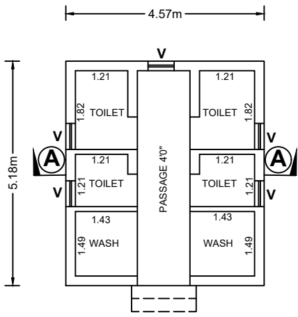
. PLAN OF TOILET.
