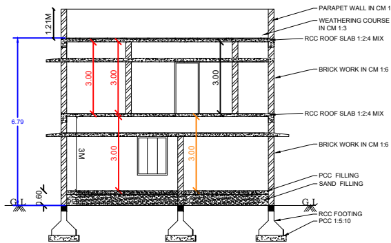
SECTION ON S-R
