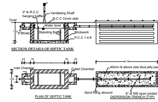
DETAILS OF SEPTIC TANK & DISPERSION TRENCH
