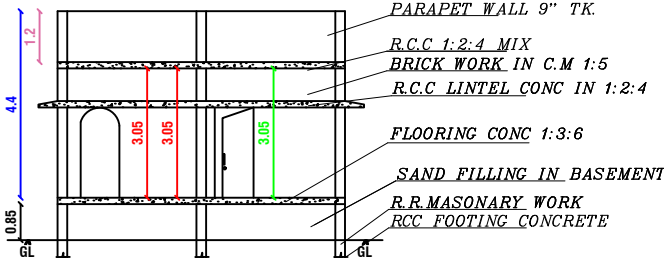
SIDE SECTION "AA"
