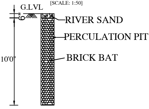
PERCOLATION PIT
