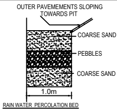
RAIN WATER PERCOLATION BED
