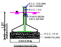
FOUNDATION DETAIL
