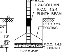
FOUNDATION DETAIL
