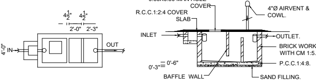
SEPTIC TANK DETAIL
