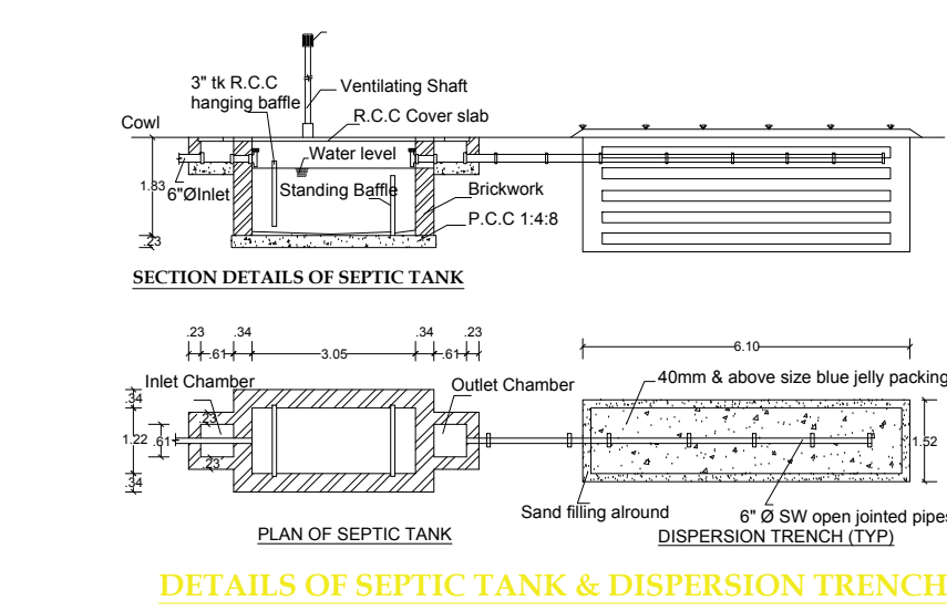
DETAILS OF SEPTIC TANK & DISPERSION TRENCH
