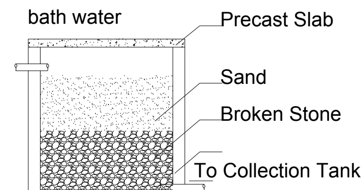
Section of Filter Unit
