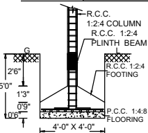
FOUNDATION DETAIL
