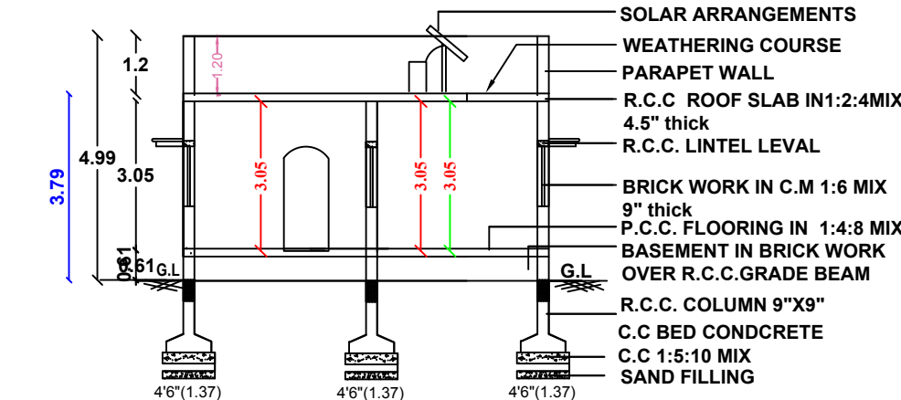
SECTION " AB "
