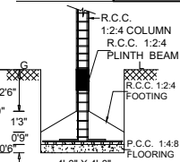
FOUNDATION DETAIL
