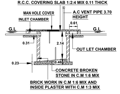
SECTION ON SEPTIC TANK . (NOT TO SCALE)
