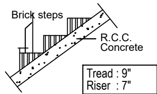
STAIRCASE DETAILS
