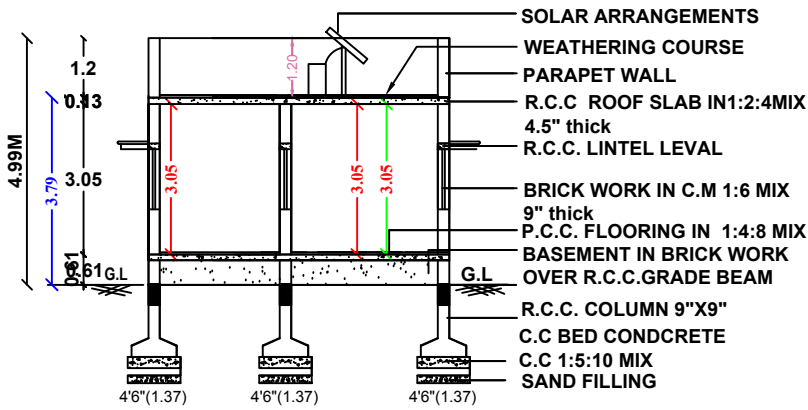
SECTION " AB "
