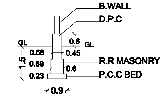
FOUNDATION DETAILS
