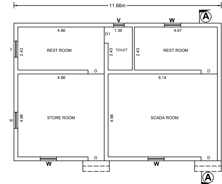
PLAN OF SCADA ROOM,STORE ROOM & REST ROOM
