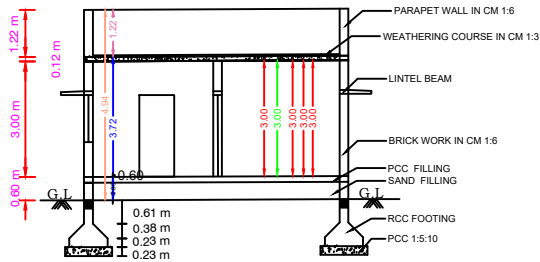
SECTION ON KA
