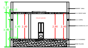
SECTION ON K-S
