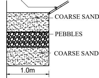
RAIN WATER PERCOLATION BED
