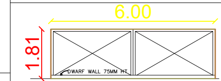
MAIN GATE
