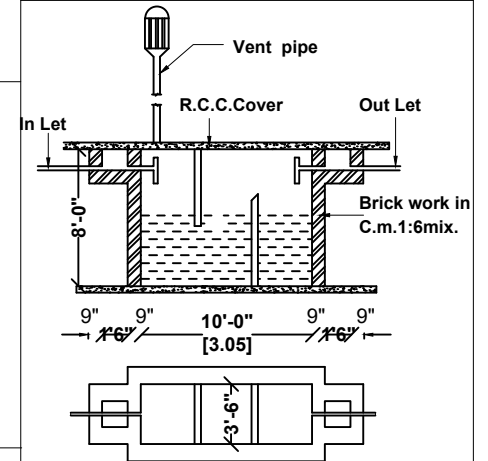
SEPTIC TANK DETAILS (NOT TO SCALE)
