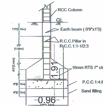
FOUNDATION DETAILS
