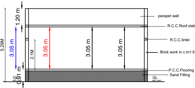
SECTION-"SR"
