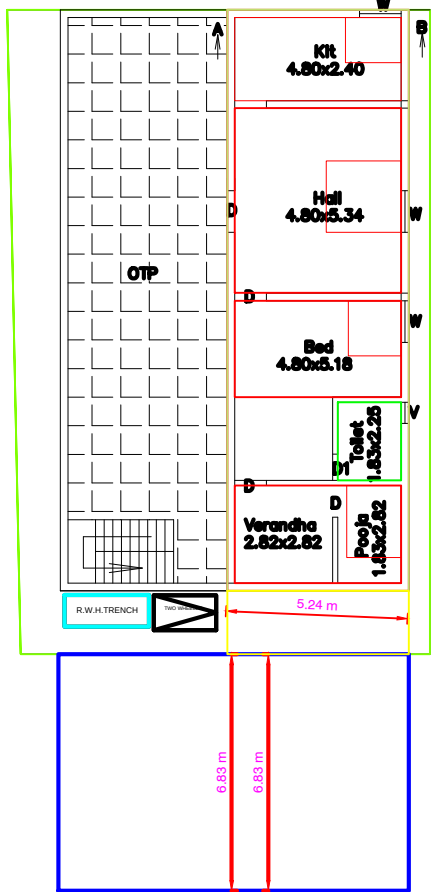
Firstfloor(Add.)
