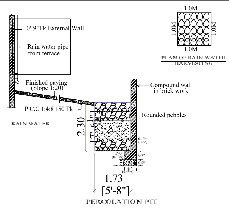
PERCOLATION PIT
