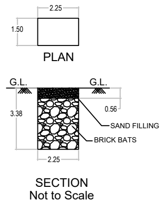
RAINWATER HARVEST PIT DETAILS
