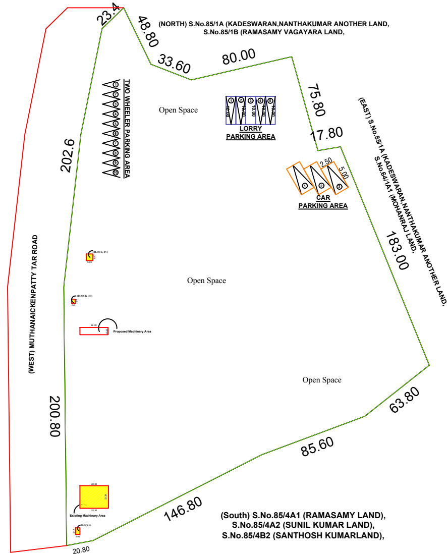
SITE PLAN
