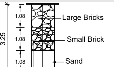
SECTION OF RAIN WATER COLLECTION PITS. (NTS)
