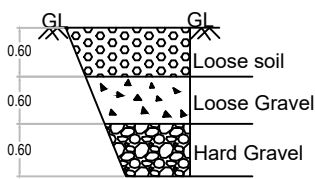
TRIAL PIT (Not To Scale)
