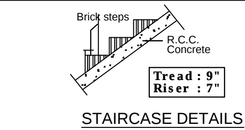
STAIRCASE DETAILS
