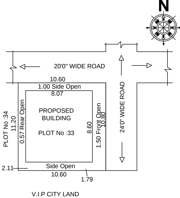
KEY PLAN
