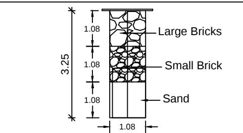
SECTION OF RAIN WATER COLLECTION PITS (NTS)
