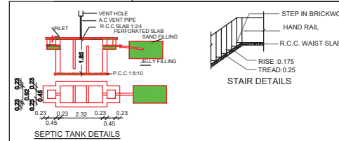
SEPTIC TANK DETAILS
