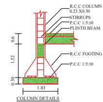
COLUMN DETAILS
