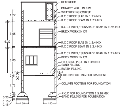
SECTION ON-AA
