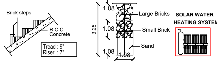
STAIRCASE DETAILS SECTION OF RAIN WATER
