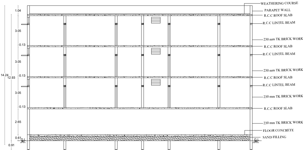
SECTION ON "BK"
