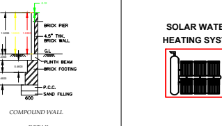
FOUNDATION DETAIL
