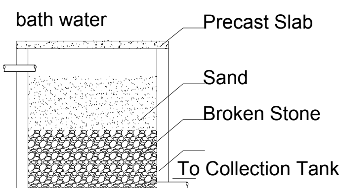
Section of Filter Unit
