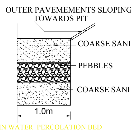
RAIN WATER PERCOLATION BED
