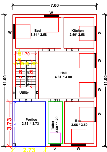
PLAN - PROPOSED GROUND FLOOR
