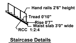
Staircase Details
