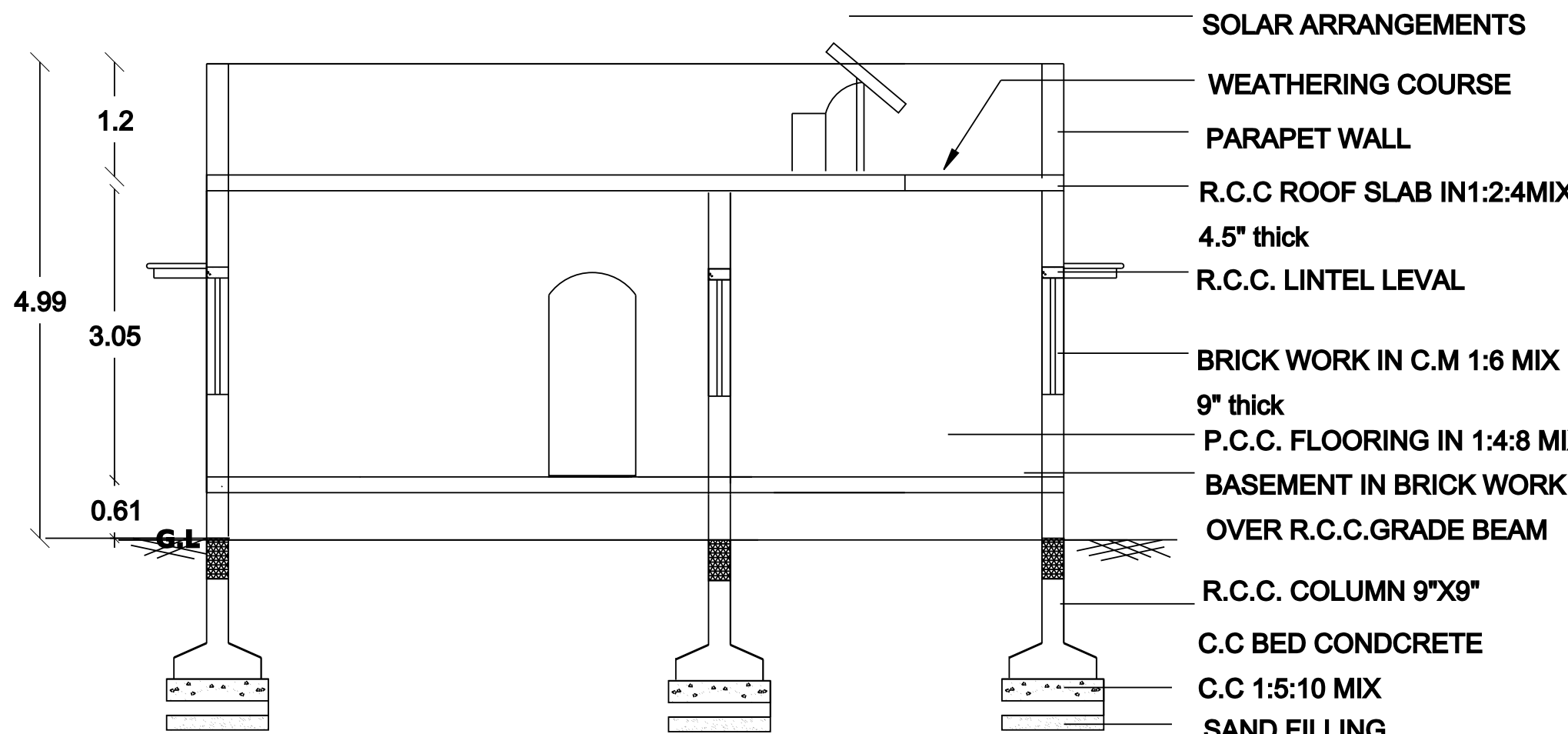
SECTION " AB "
