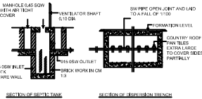
SECTION OF SEPTIC TANK
