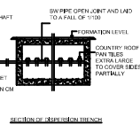
SECTION OF DISPERSION TRENCH
