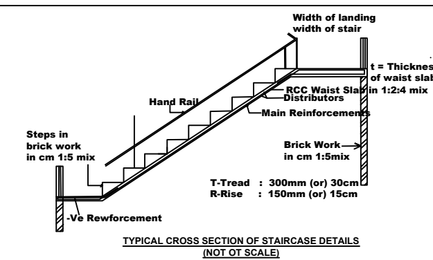
TYPICAL CROSS SECTION OF STAIRCASE DETAILS (NOT OT SCALE)
