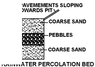
WATER PERCOLATION BED
