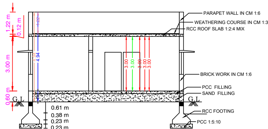
SECTION OF KA
