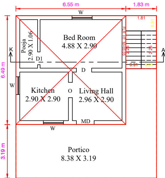
EXISTING AND ADDITIONAL GROUND FLOOR PLAN
