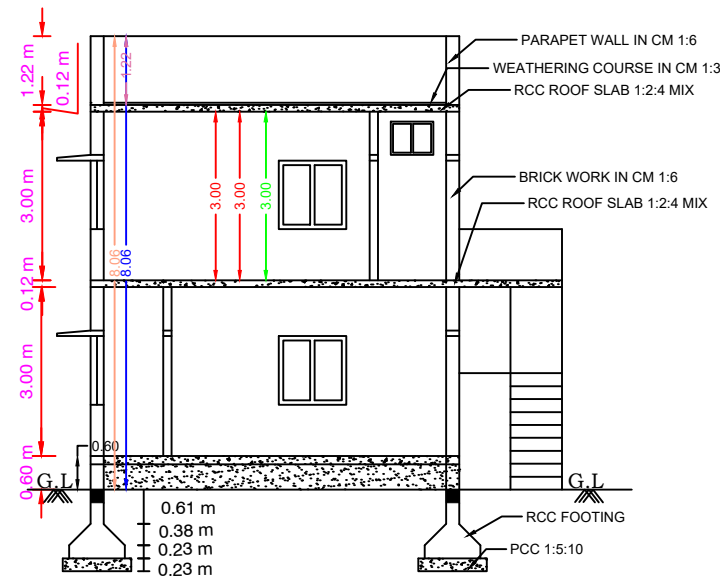
SECTION ON KA
