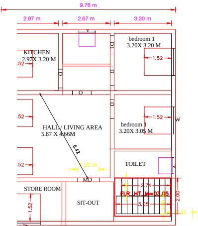
EXISTING FIRST FLOOR PLAN
