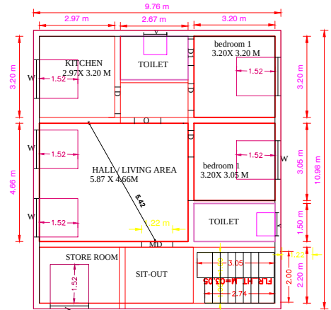
POP. SECOND FLOOR PLAN
