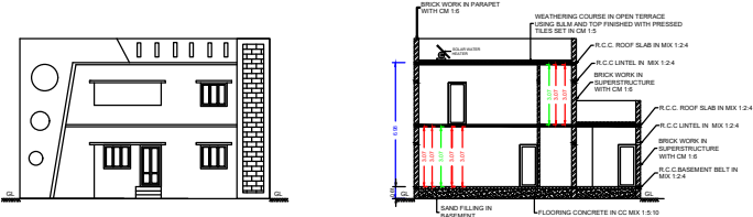
FRONT ELEVATION
