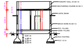
SECTION ON KA
