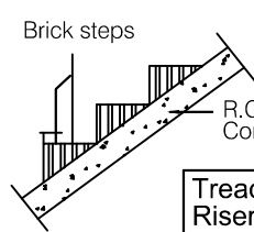
STAIRCASE DETAILS
