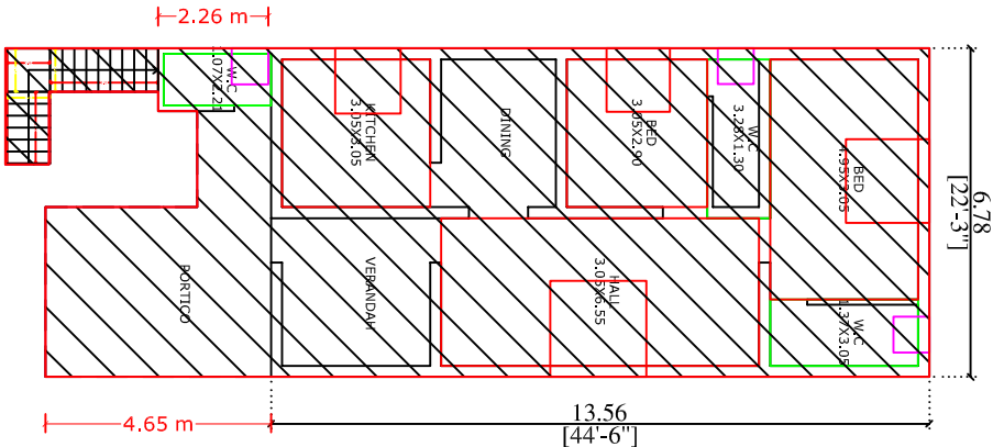
EXISTING GROUND FLOOR
