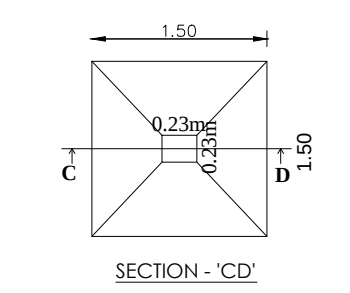
Isolated Footing -A (1.50X1.50) (Not to Scale)
