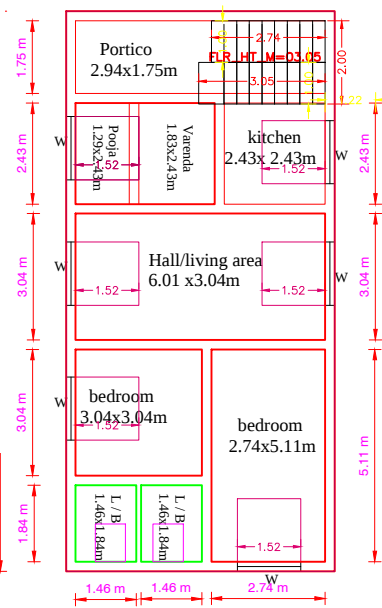
PROP. FIRST FLOOR PLAN
