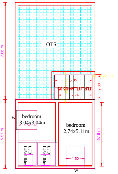
PROP. SECOND FLOOR PLAN
