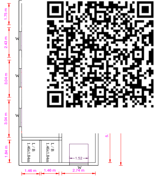
EX.GROUND FLOOR PLAN
