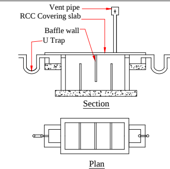
SECTION - 'CD'
