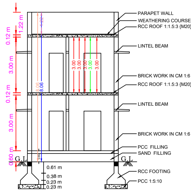
SECTION ON KA
