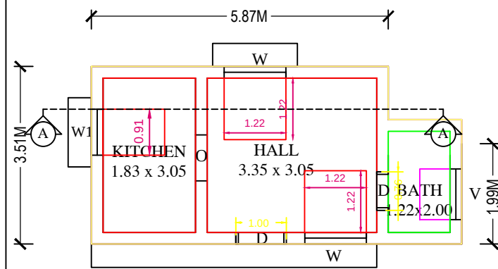
PRO.GOUND FLOOR PLAN FACING NORTH
