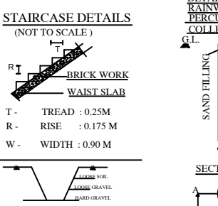
STAIRCASE DETAILS (NOT TO SCALE) DETAILED PLAN OF RAINWATER COLLECTION AND DISTRIBUTION (NOT TO SCALE)
