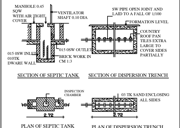
SECTION OF SEPTIC TANK SECTION OF DISPERSION TRENCH
