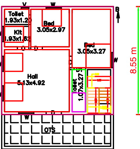
FIRST FLOOR PLAN(Pro.)
