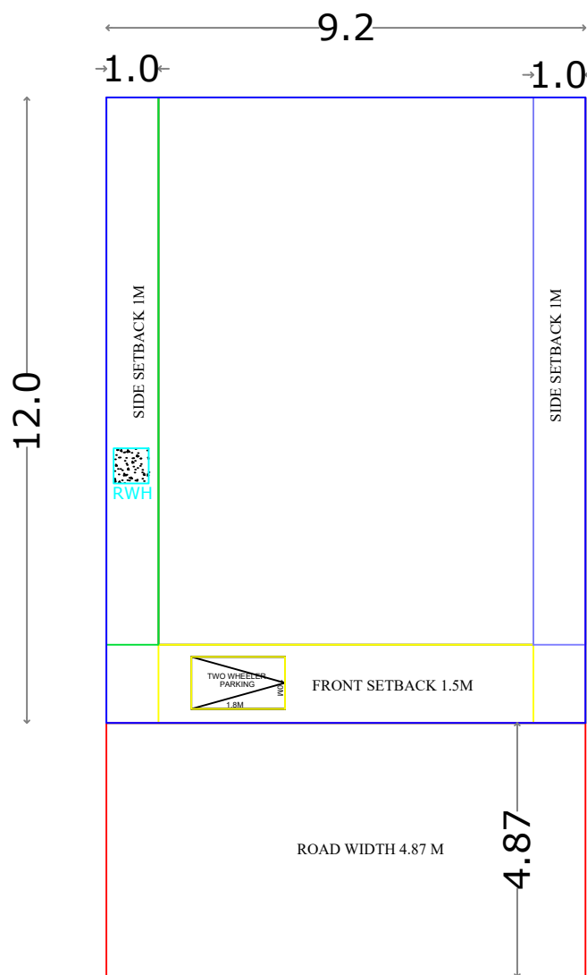
SITE PLAN
