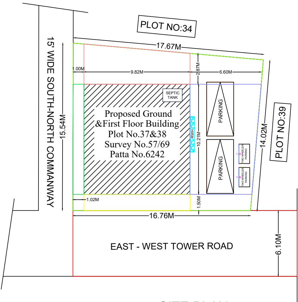
SITE PLAN
