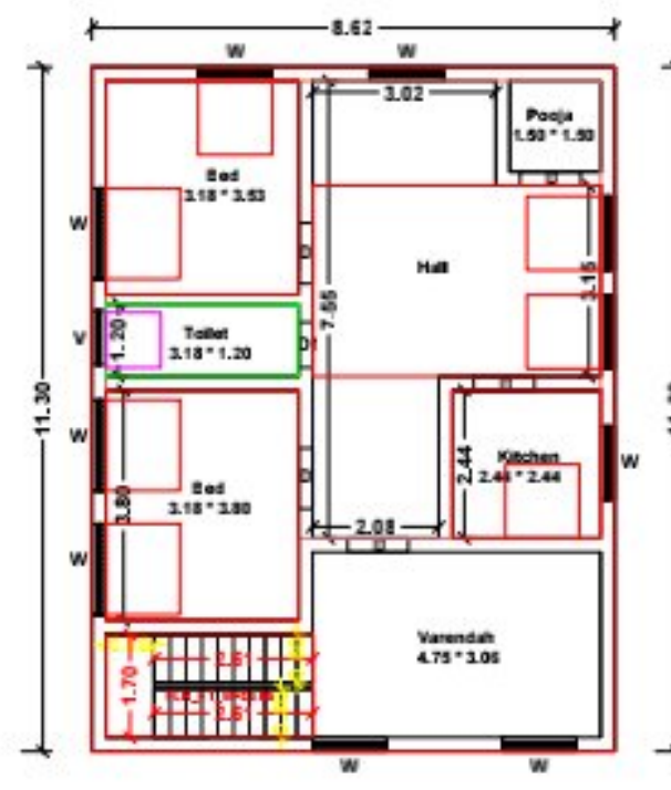
PLAN - PROPOSED FIRST FLOOR
