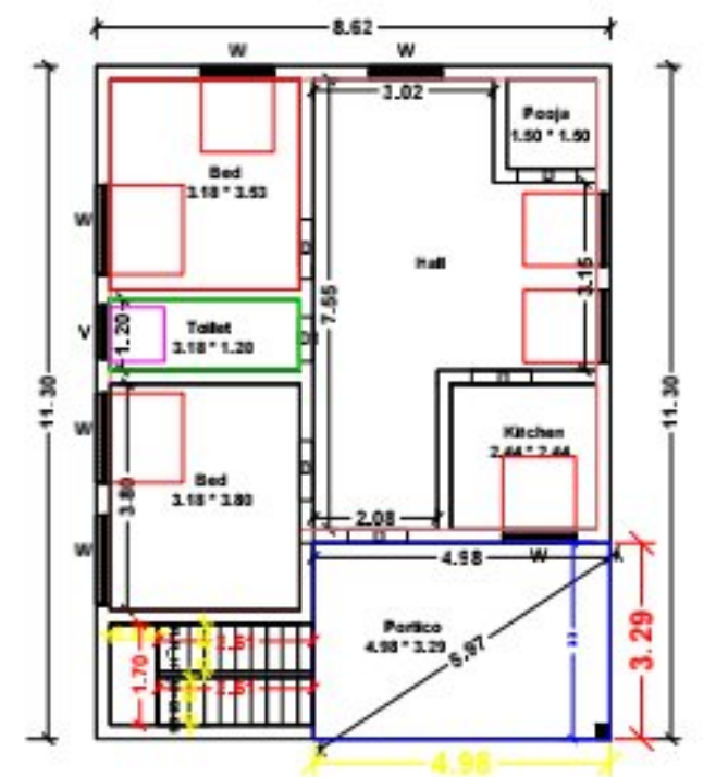
PLAN - PROPOSED GROUND FLOOR
