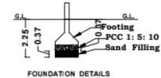
FOUNDATION DETAILS
